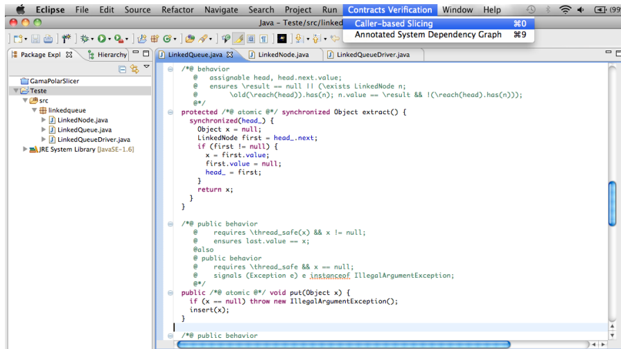
Fig. 2. Eclipse interface with the GammarPolarSlicer plugin prototype
