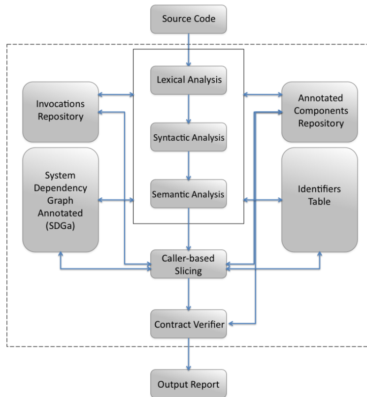
Fig. 1. GammaPolarSlicer Architecture
