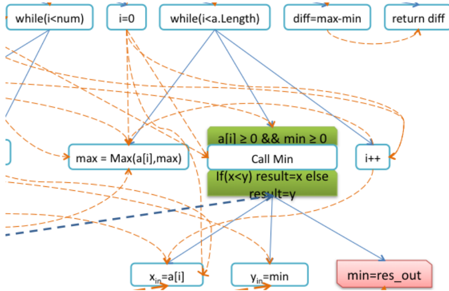
Fig. 3. Example of an Annotated System Dependency Graph
